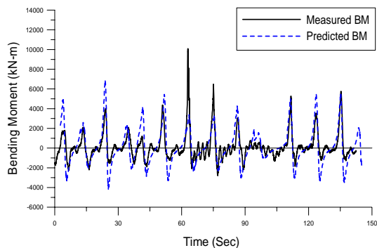
Fig. 4 Comparison of measured and predicted bending moment at mudline
