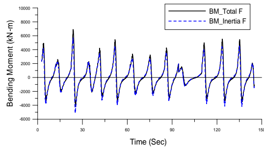
Fig. 5 Comparison of total bending moments and bending moments due to only inertia forces in campaign H_s = 6.1 m
