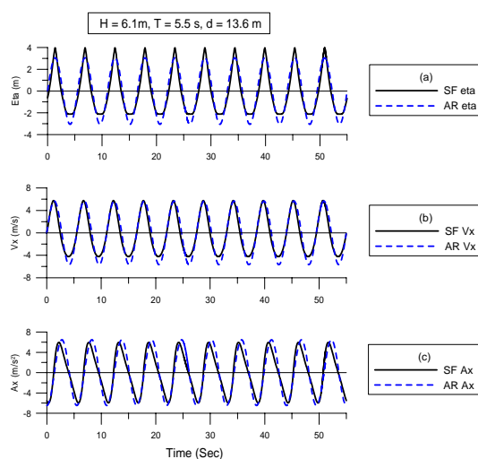
Fig. 1 Comparison Wave Profiles and Kinematics of Stream function and Airy theory at 8.76 m from bottom
