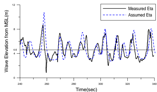
Fig. 3 Comparison between measured wave profile and that used for wave-by-wave calculations (Hs= 6.1m)
